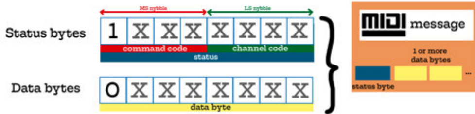
Figure 2.8: MIDI byte types
